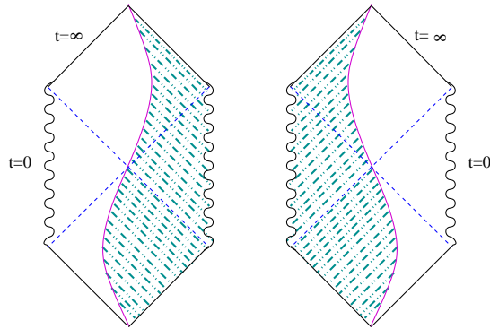
Figure 1: Graphical representation of a brane-world embedded in an S-brane background.
