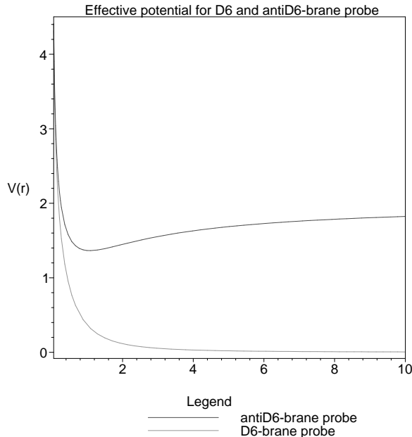
Figure 7: The effective potential for the radial motion of the brane centre-of-mass.
