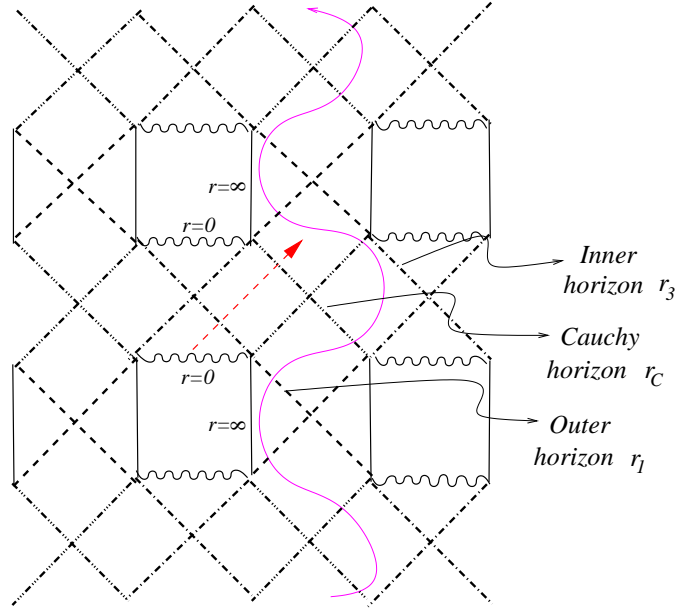
Figure 4: Penrose diagram for solution (3.43). Notice the presence of space-like naked singularities, from which signals can affect brane physics. As a consequence of these naked singularities, Cauchy horizons are present.
