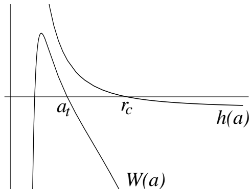
Figure 2: Plot of the potential W of (3.23) and of the metric function h in (3.11). Writing \rho_m = c a^{-3(1+\omega)} , we choose \omega = 1/3 , \xi = 3 , \lambda = 1 , \Lambda = 10^{-4} , c = 1 . Notice that we have a bounce around the turning point represented by a_t , the minimum value for the scale factor, that corresponds to a zero for W . This point is inside the Cauchy horizon, which is labeled by r_C .
