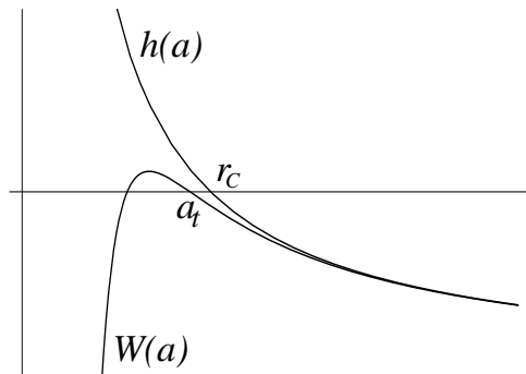
Figure 3: Effective potential for the dilatonic model described in eq. (3.36). We choose \sigma = 1 , \Lambda_2 = 33 , \lambda = 3.8 . The metric function h(a) , given in (3.27), is also included.
