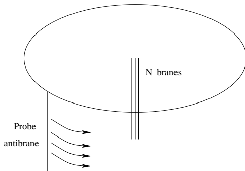
Figure 6: Branonium is the bound state of an anti-brane orbiting a set of source branes.
