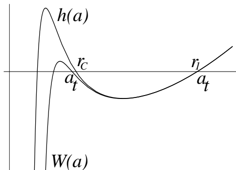
Figure 5: Effective potential (3.48), for the charged dilatonic model. For the parameters, we choose M = 10^{-2} , \Lambda_3 = Q = 1.6 , \lambda = 0.06 . The metric function h(a) , given in (3.43), is also included.
